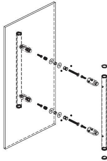
ISO EXPLODED VIEW-2
